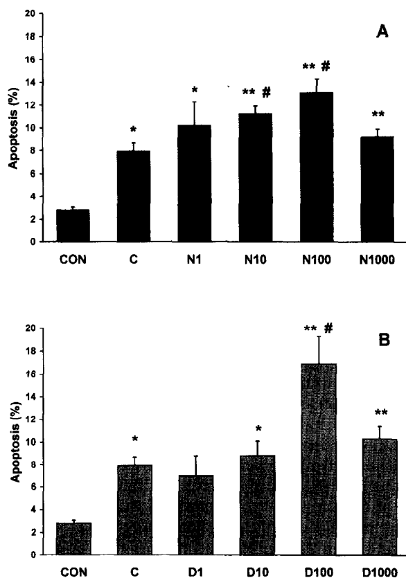
Fig. 1. Effects of cytomix, neopterin and 7,8-dihydroneopterin on apoptosis in L2 cells. L2 cells were incubated for 24 h with the cytomix (C; 100 U/ml IFN- \gamma plus 500 U/ml TNF- \alpha ), with neopterin (N; 1 \mu M, 10 \mu M, 100 \mu M, 1000 \mu M; A) or with 7,8-dihydroneopterin (D; 1 \mu M, 10 \mu M, 100 \mu M, 1000 \mu M; B). Apoptotic cell death is characterized by measurement of intranuclear contents of DNA by FACS analysis as described in Section 2. Data are shown as mean values \pm S.E.M. ( n=7 ). * P<0.05 and ** P<0.01 as compared with untreated control cultures (CON), # P<0.05 as compared with the cytomix (C).
