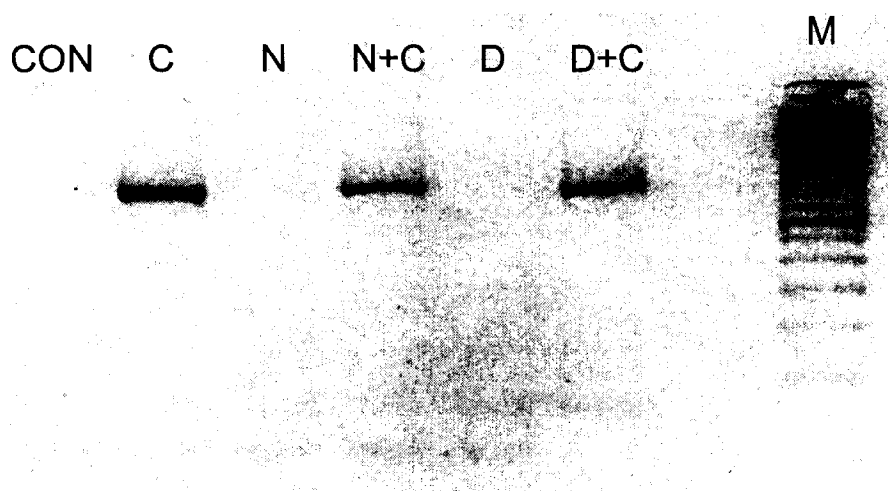
Fig. 4. Qualitative PCR analysis of iNOS mRNA expression detected as iNOS cDNA (fragment size: 498 bp) following 9 h incubation of L2 cells with the cytomix (C; 100 U/ml IFN- \gamma and 500 U/ml TNF- \alpha ), 100 \mu M neopterin (N), 100 \mu M neopterin plus cytomix (N+C), 100 \mu M 7,8-dihydroneopterin (D), and 100 \mu M 7,8-dihydroneopterin plus cytomix (D+C). Lane CON shows the results of a control experiment in untreated cells. Lane M indicates the molecular mass marker (50 bp ladder). Results are representative of three different experiments.
