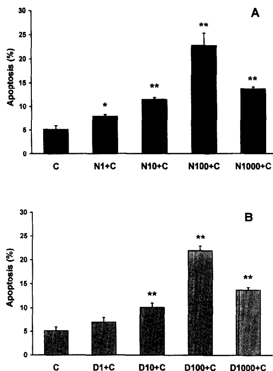
Fig. 2. Apoptotic cell death induced by the coincubation of cytomix with neopterin and cytomix with 7,8-dihydroneopterin. A: L2 cells were incubated for 24 h with the cytomix (C; 100 U/ml IFN- \gamma and 500 U/ml TNF- \alpha ), 1 \mu M neopterin plus the cytomix (N1+C), 10 \mu M neopterin plus cytomix (N10+C), 100 \mu M neopterin plus cytomix (N100+C) or 1000 \mu M neopterin plus cytomix (N1000+C). B: L2 cells were incubated for 24 h with the cytomix, 1 \mu M 7,8-dihydroneopterin plus the cytomix (D1+C), 10 \mu M 7,8-dihydroneopterin plus cytomix (D10+C), 100 \mu M 7,8-dihydroneopterin plus cytomix (D100+C) or 1000 \mu M 7,8-dihydroneopterin plus cytomix (D1000+C). Apoptosis is characterized by measurement of intranuclear contents of DNA by FACS analysis as described in Section 2. The percentage of apoptotic cells in untreated controls was subtracted from treated cell cultures. Data are presented as mean values \pm S.E.M. ( n=7 ). * P<0.05 and ** P<0.01 as compared with the cytomix, # P<0.01 as compared with the cytomix (C).
